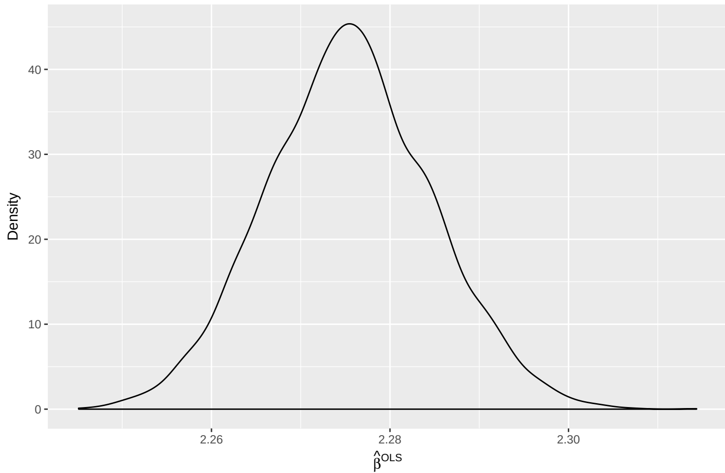
Density of OLS Estimator with N = 10000
